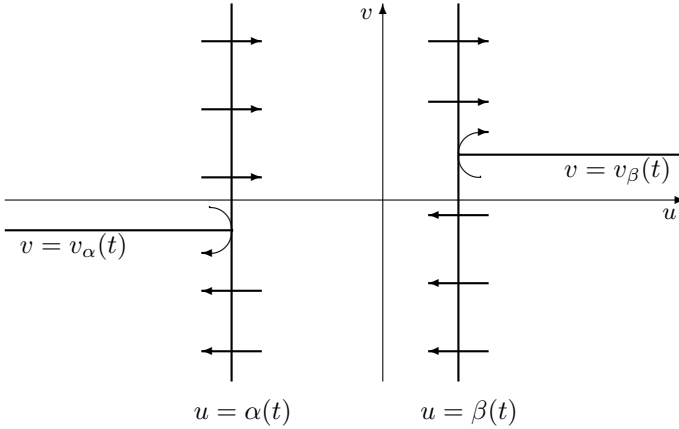
FIGURE 1. A visual illustration of the above definitions from a dynamical point of view. Horizontal arrows represent the relative velocity u' of solutions of system (5) compared with \alpha' and \beta' , as stated in (7) and (9). Curved arrows indicate the essence of conditions (8) and (10), comparing v' with v'_\alpha and v'_\beta .
