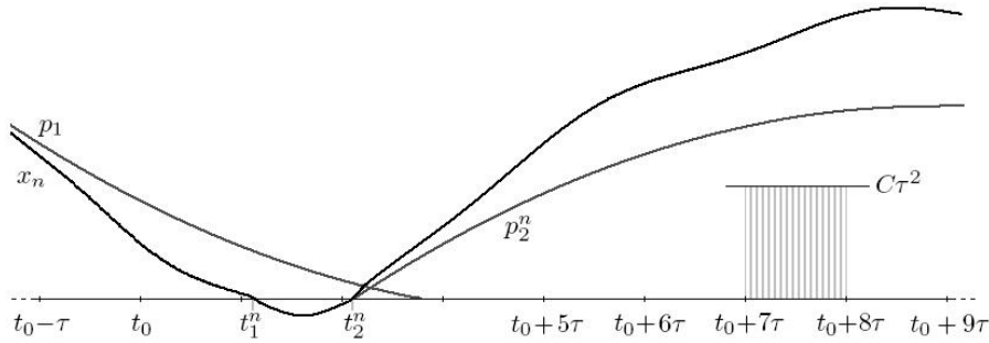
Figure 2: The figure shows how the two parabolas p_1 and p_2^n control the solution x_n . In the interval [t_0 + 7\tau, t_0 + 8\tau] , one has that x_n(t) is greater than C\tau^2 .
