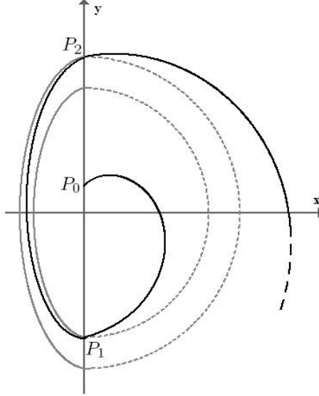
Figure 1: It is shown how to construct the first lap of the spiral \gamma_n , in black. In \Pi^+ two half-balls are drawn, in dotted grey, and in \Pi^- two branches of two orbits of equation (12), in grey. These branches locate two particular examples of the set E_r^n .
